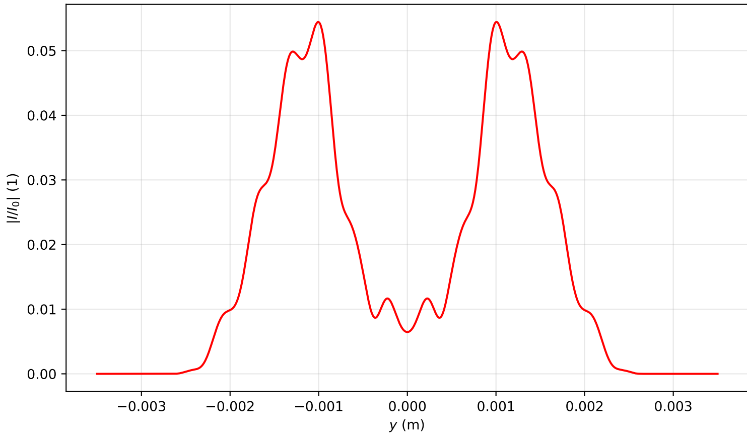
Intensity profile I(x=0, y, z=3.821)/I_0 , P_{in}=6.0P_{cr} , artificial time
